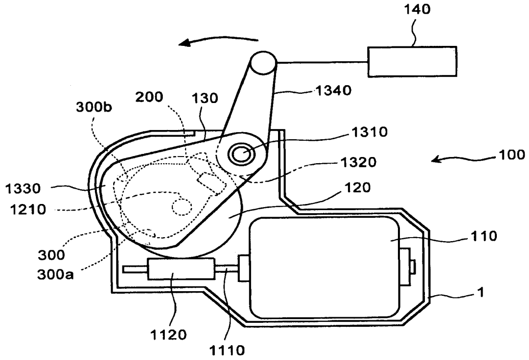
FIG.8 PRIOR ART
